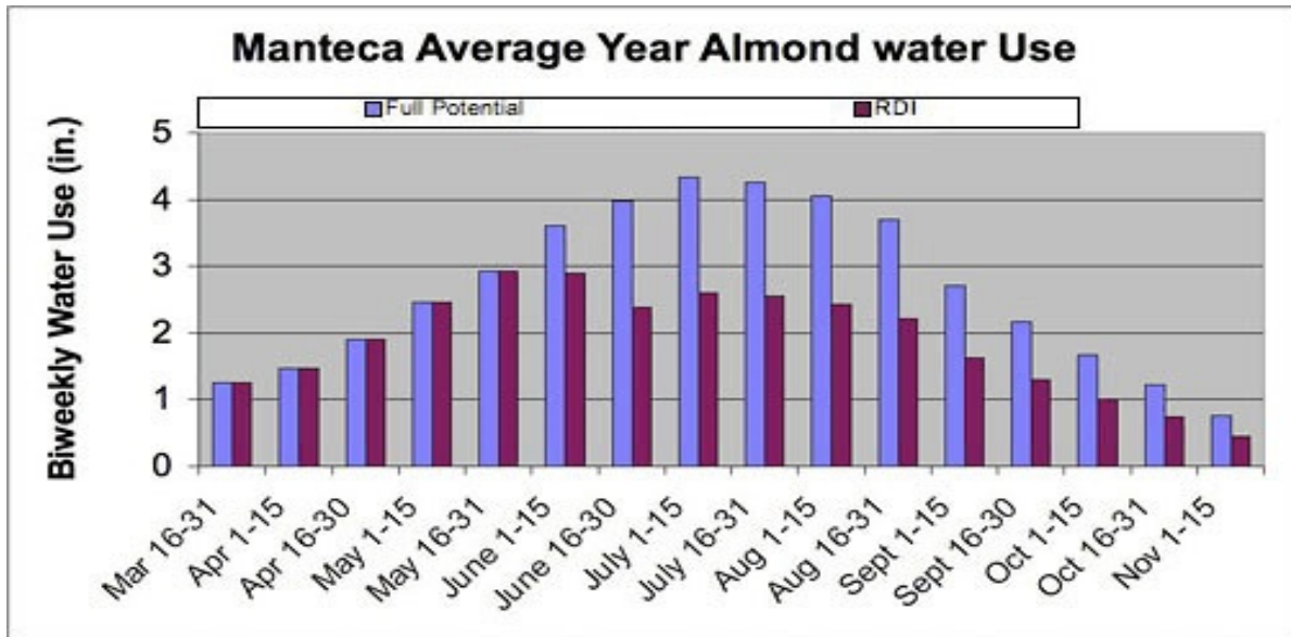
Figure 1: Seasonal water use for an almond orchard in Manteca, CA.
